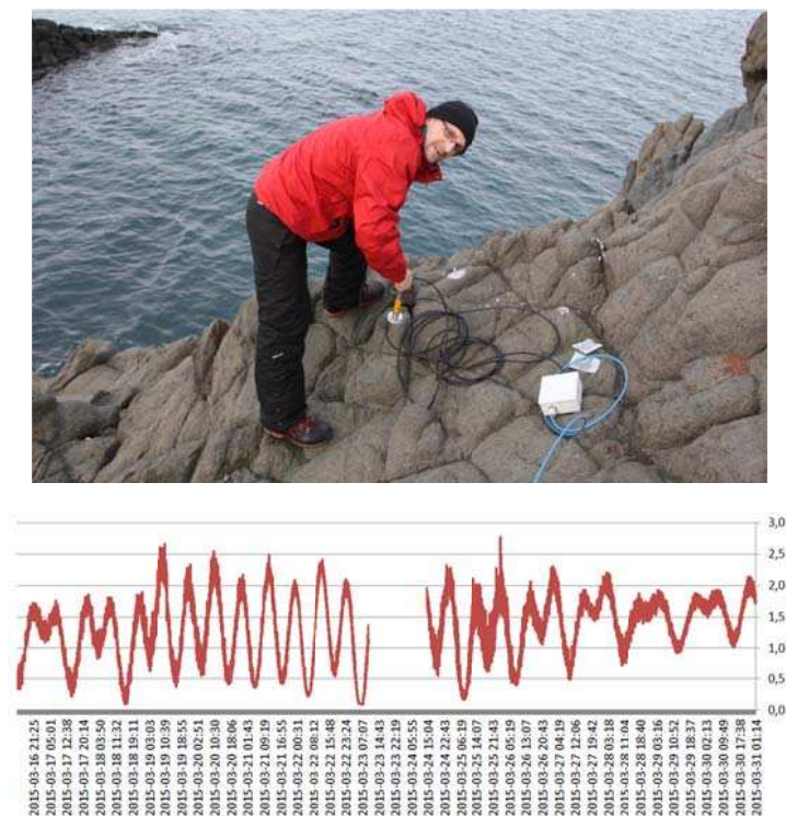
Fig. 21. Mounting of prototypical measurement system based on a hydrostatic probe and a graph representing water level changes in Admiralty Bay registered during the time of expedition
