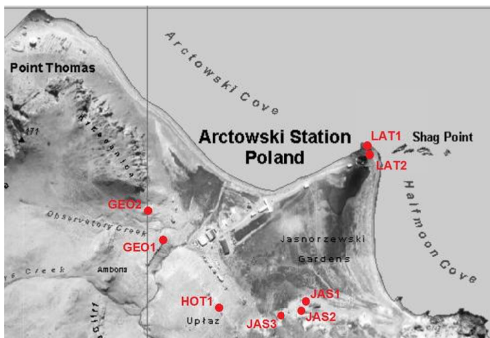
Fig. 20. Geodetic surveying network around Arctowski Station on King George Island (Pasik et al., 2016).
